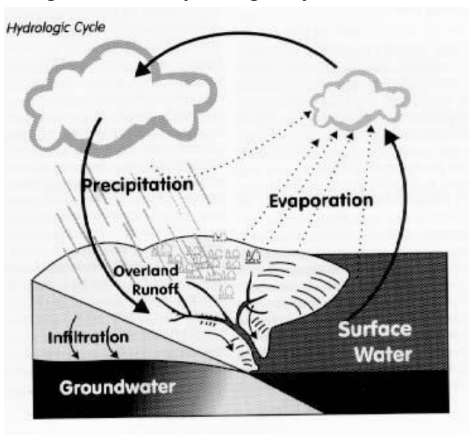
Figure 1. The Hydrologic Cycle
