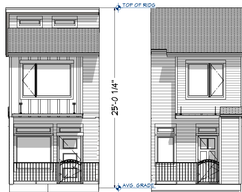
2 STORY FRONT
