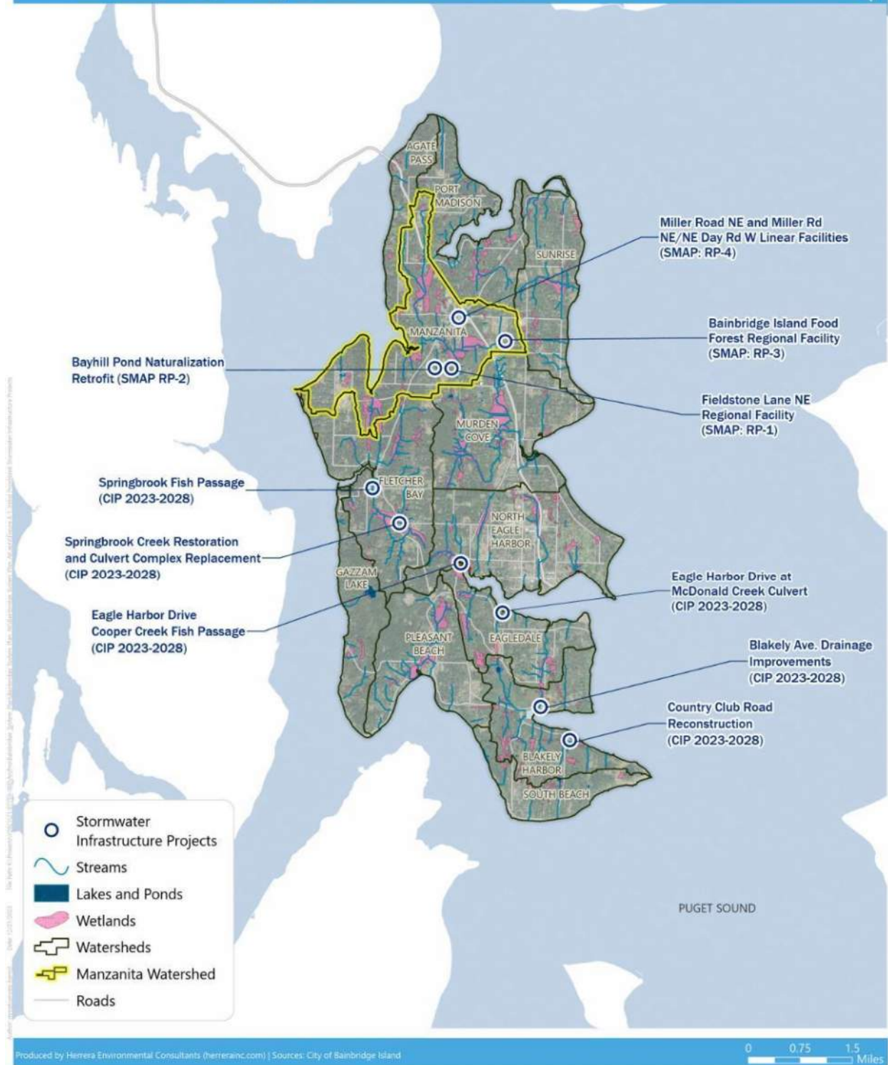
Figure 4-1. Substantial Stormwater Infrastructure Improvement Projects Identified for Prioritization.
