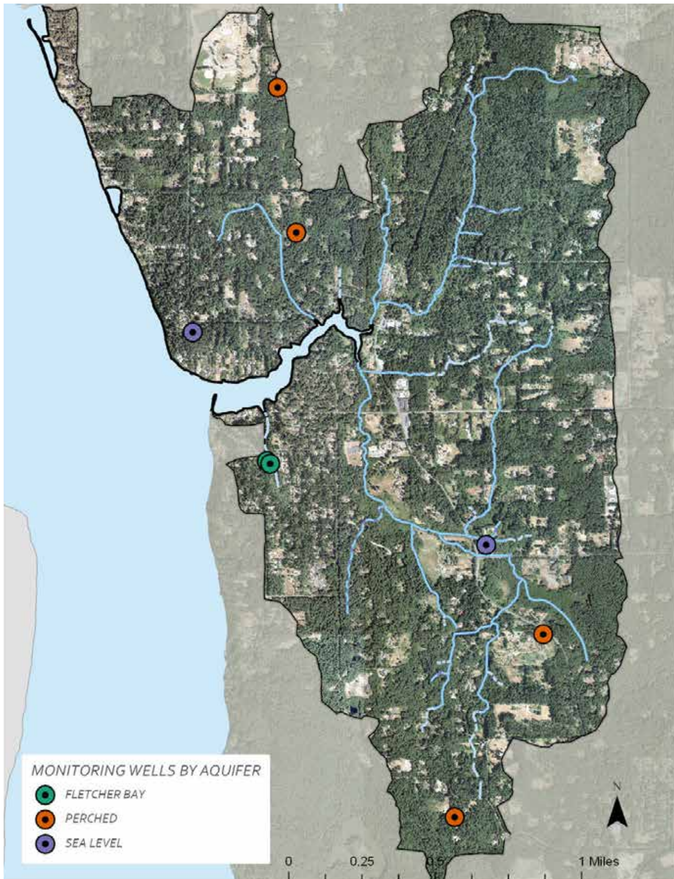
Figure 9. Fletcher Bay Watershed monitoring wells by location and aquifer
